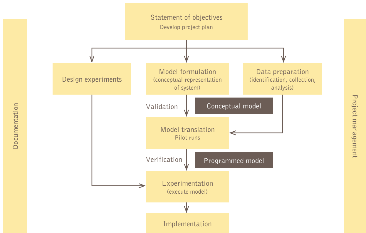
Figure 1: The simulation modeling and analysis process
